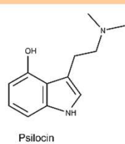
Psilocin
