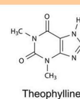
Theophylline
