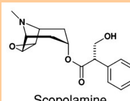
Scopolamine
