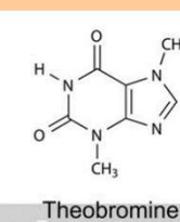
Theobromine
